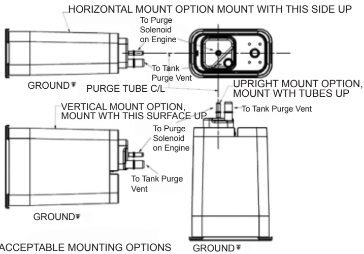
ACCEPTABLE MOUNTING OPTIONS FOR PROPER LIQUID TRAP FUNCTION
